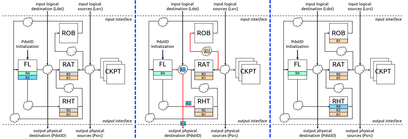
Figure 2. Walkthrough example demonstrating how a bug in write-enable signal of the RAT leads to leakage and duplication.
