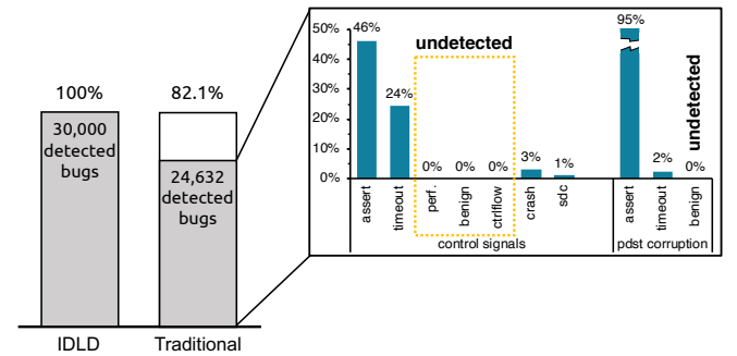
Figure 9. Bug detection capability of IDLD and traditional end-of-test checking post-silicon validation.
