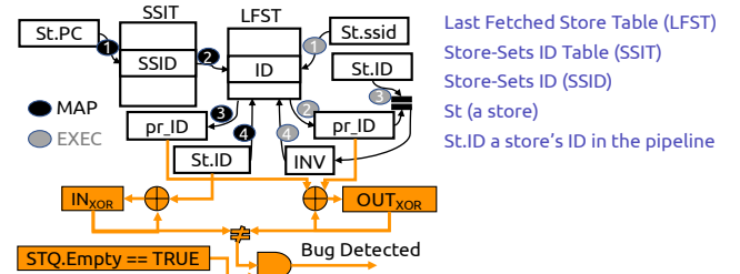
Figure 7. IDLD use case for MDP. Black circles represent the MDP flow for a store instruction at the map stage and the grey circles the flow when the store address is known at execute.
