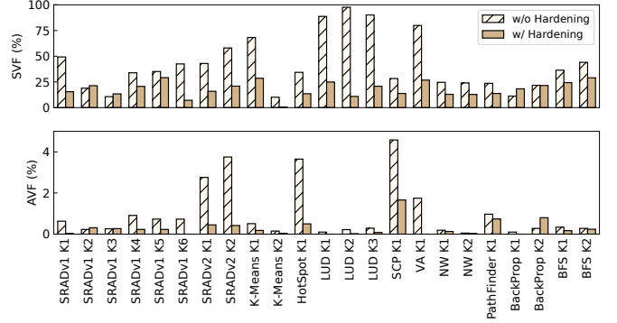
Fig. 2. AVF and SVF of hardened applications.
