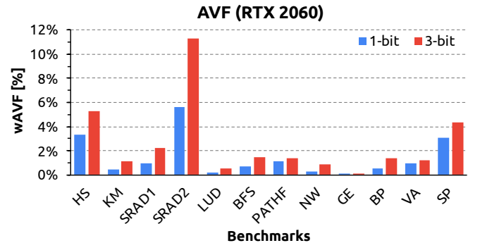
Fig. 6. Weighted AVF for single-bit (blue color) vs. triple-bit (red color) fault injections for RTX 2060 and for twelve benchmarks.
