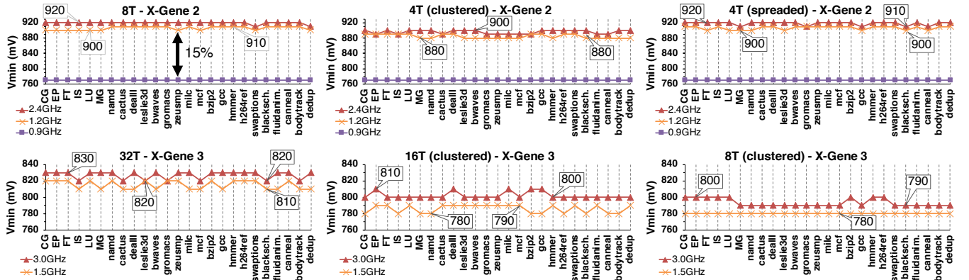
Figure 3. The complete V_{min} characterization results. The top diagrams show the X-Gen 2 safe V_{min} points for all benchmarks with 8 and 4 threads in 2.4, 1.2 and 0.9 GHz. The bottom diagrams show the X-Gen 3 safe V_{min} points for all benchmarks with 32, 16 and 8 threads in 3.0 and 1.5 GHz.
