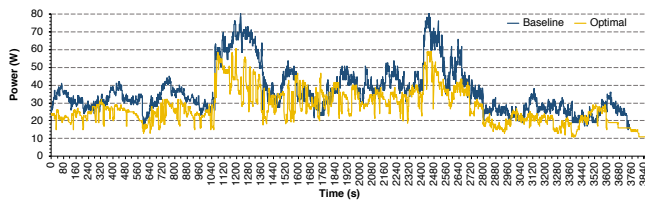
Figure 14. Average power for the Baseline and the Optimal configurations in X-Gen 3 during 1-hour execution.
