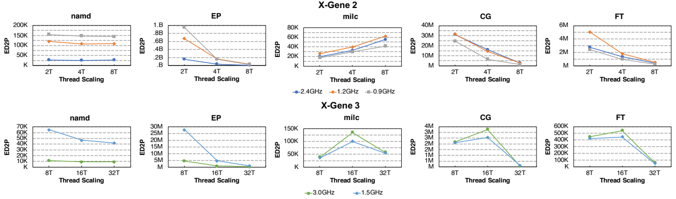
Figure 12. Energy Delay Squared Product (ED2P) for 8, 4, and 2 threading options for 3 different frequencies (2.4GHz, 1.2GHz, 0.9GHz) of X-Gene 2 (top) and 32, 16, and 8 threading options for 2 different frequencies (3GHz, 1.5GHz) of X-Gene 3 (bottom).
