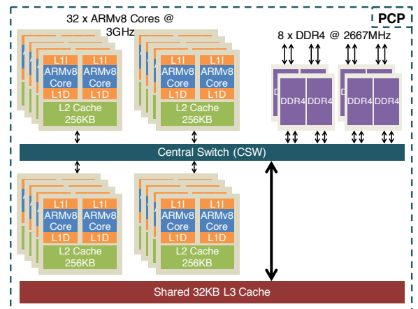
Figure 1. X-Gene 3 block diagram.
