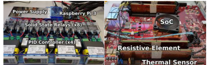
Fig. 3: a) X-Gene 2 with the thermal adapters, b) Temperature controller board.
