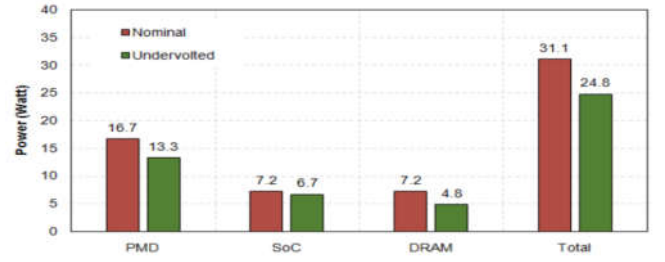
Fig. 9: Power consumption per domain for nominal and undervoltted operation
