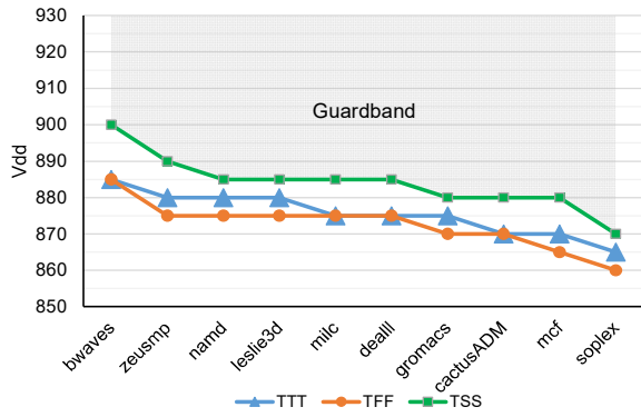
Fig. 4: Vmin results at 2.4 GHz for 10 SPEC2006 programs on 3 different X-Gene 2 chips (TTT, TFF, TSS)
