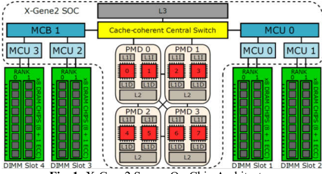
Fig. 1: X-Gene2 Server-On-Chip Architecture
