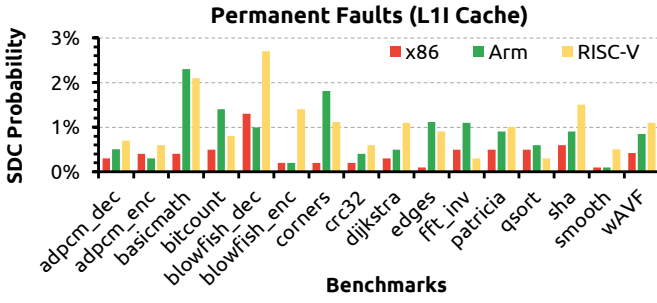
Fig. 3. SDC probability due to permanent faults in L1 instruction cache [46].
